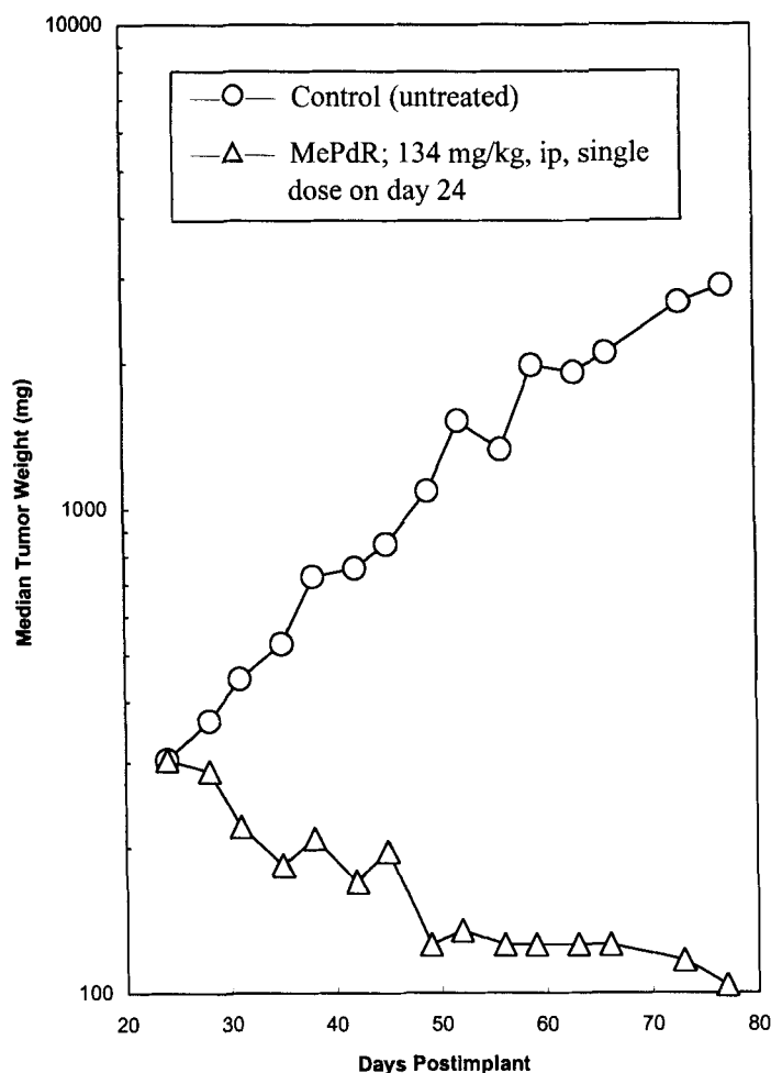
FIG. 1. Response of Subcutaneous D54 CNS Tumors Transfected with E. coli PNP to Treatment with MePdR.
